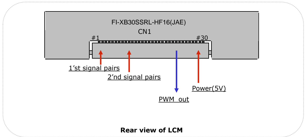
FIG. 4 Connector diagram
